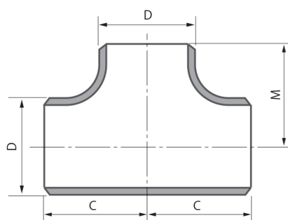
STRAIGHT TEE
